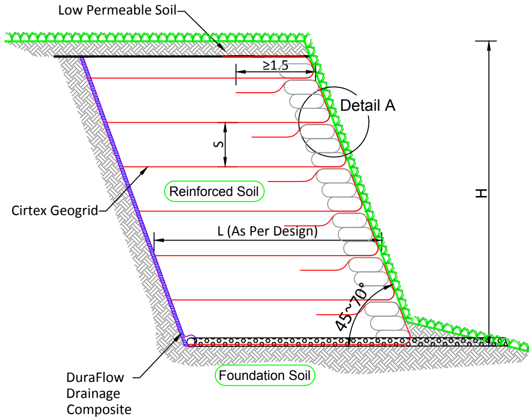
DuraGreen Typical Cross Section
