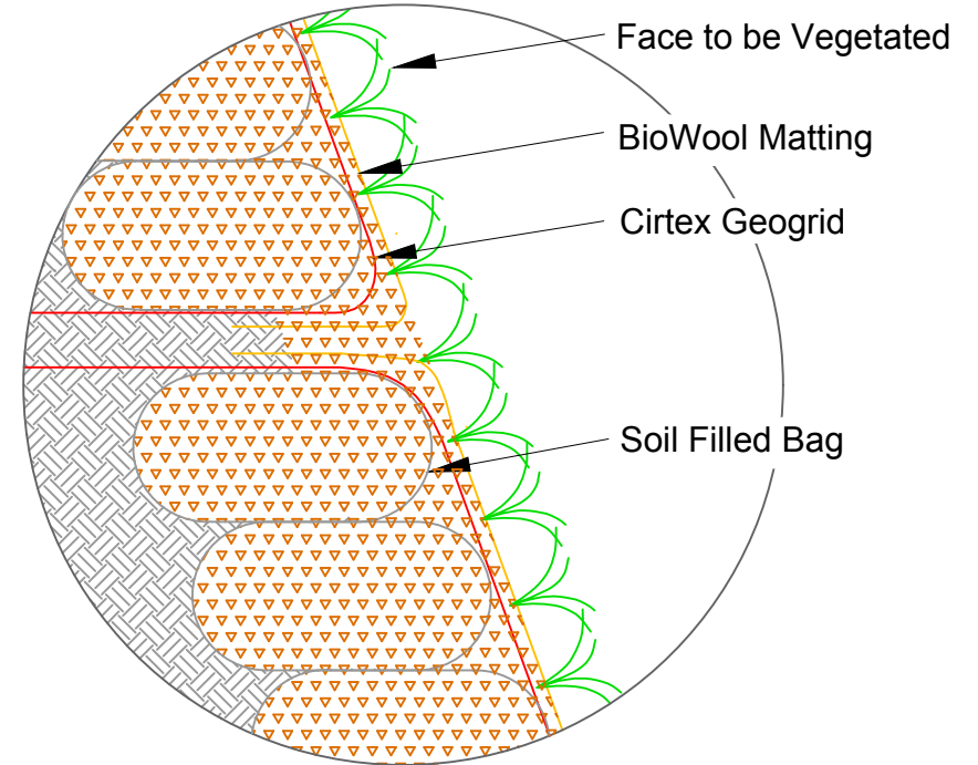
Detail A: DuraGreen Facing System
